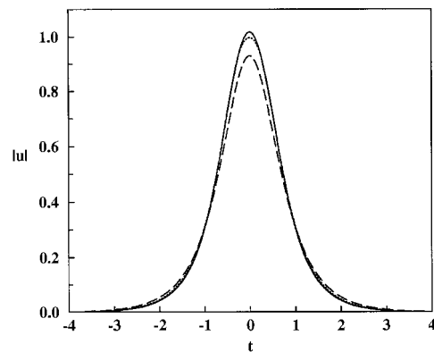
Figure 2. Comparison of pulse shapes obtained with the numerical (solid curve), analytical (dotted curve) and path-averaged NLS (dashed curve) solutions. Here \ddot{\beta}_2 - \ddot{\beta}_1 = 1.82 \text{ ps}^2/\text{km} .
