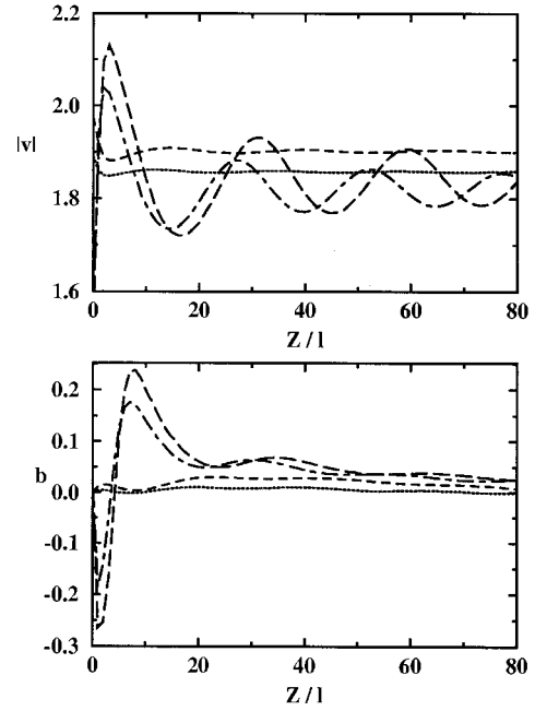
Figure 7. Graphs of the peak pulse amplitude |v(t = 0)| and the chirp parameter b measured stroboscopically at the analytically-predicted GVD-independent chirp-free points. The launch point is either a chirp-free point (Case I: dotted lines; Case II: dashed lines) or the beginning of the normal dispersion segment (Case I: dot-dashed lines; Case II: long dashed lines). Here Z/l = z/\varepsilon . The parameters for Cases I and II are described in the text.
