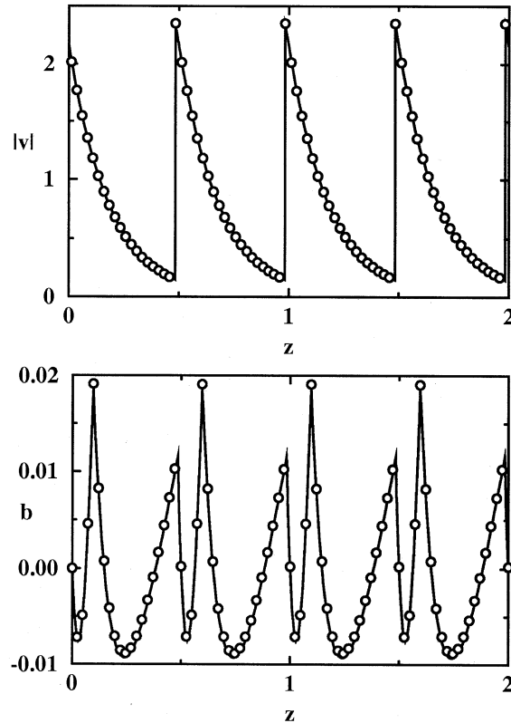
Figure 5. Evolution of the peak pulse amplitude |v(t=0)| and the chirp parameter b (circles: numerical results; solid lines: asymptotic predictions). The parameters are described in the text.
