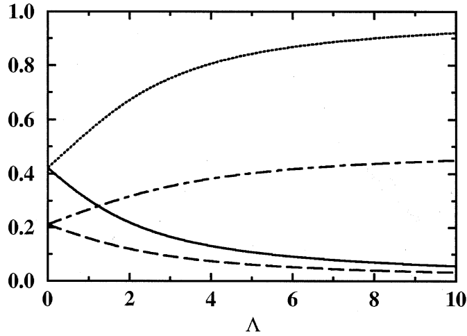
Figure 4. The magic fractions and the locations of the corresponding GVD-independent chirp-free points as functions of the loss coefficient \Lambda . The fraction \zeta_1 (solid line) and the distance \zeta_a (dashed line) amplifier, while \zeta_2 (dotted line) and \zeta_b (dot-dashed line) are plotted when the chirp-free point is on the fiber segment before the amplifier.
