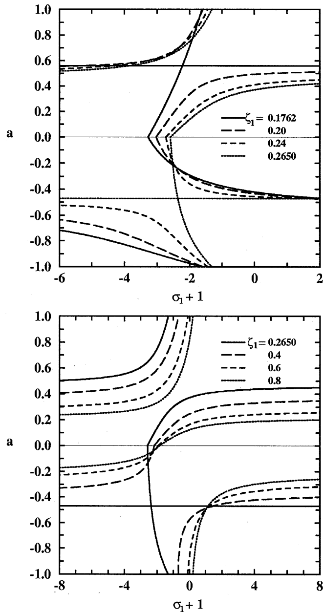
Figure 3. Locations of the chirp-free points within a dispersion map period. The distance between a chirp-free point and the amplifier is normalized by the length of the segment on which the chirp-free point lies and positive (negative) values of the normalized distance a correspond to chirp-free points on the segment after (before) the amplifier. Here the loss parameter is \Lambda = 2.763 .
