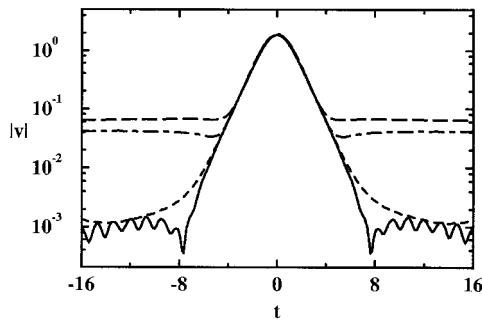
Figure 8. Pulse profiles after propagation over 82 dispersion map periods (9,840 km). The launch point is either a chirp-free point (Case I: solid lines; Case II: dashed lines) or the beginning of the normal dispersion segment (Case I: dot-dashed lines; Case II: long dashed lines). The parameters for Cases I and II are described in the text.
