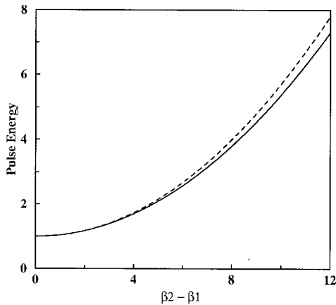
Figure 1. Comparison between the numerical (solid curve) and analytical (dashed curve) results for the soliton power enhancement due to a two-step dispersion map. The parameters are as described in the text, and the pulse energy has been normalized by -3.52\langle \ddot{\beta} \rangle / (\gamma \tau_{\text{FWHM}}) .
