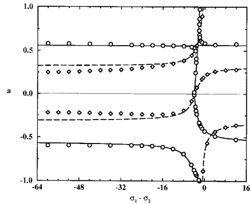
Figure 9. Comparison of numerically determined chirp-free point locations (circles: \zeta_1 = 0.1762 ; diamonds: \zeta_1 = 0.5 ) for dispersion-managed solitons with the asymptotic predictions (solid lines: \zeta_1 = 0.1762 ; dashed lines: \zeta_1 = 0.5 ). Here the normalized dispersion-map period is \varepsilon = 0.4 and the loss parameter is \Lambda = 2.763 . The parameter a specifies the chirp-free point locations and is defined in the text.
