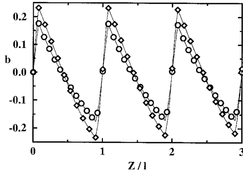
Figure 6. Evolution of the chirp parameter b in Cases I (circles) and II (diamonds) (with parameters described in the text) after unchirped power-enhanced hyperbolic-secant pulses are launched at a GVD-independent optimal launch point.
